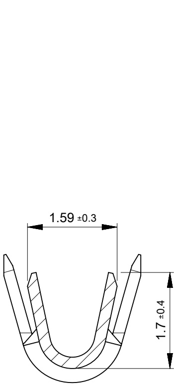
SECTION Z-Z
