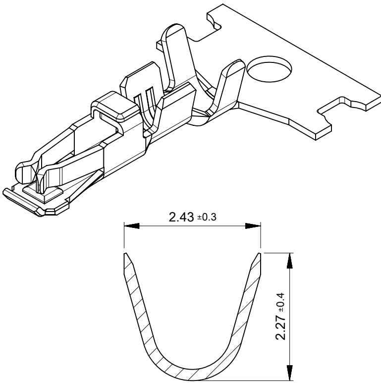
SECTION Y-Y
